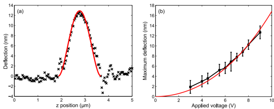
Figure 3. (a) Deflection profile versus the length of an 8.1 nm thick graphene membrane actuated at DC bias of 9 V. (b) Maximum deflection of the membrane under different DC bias voltages. Reprinted/adapted with permission from [55]. Copyright 2013, AIP.
